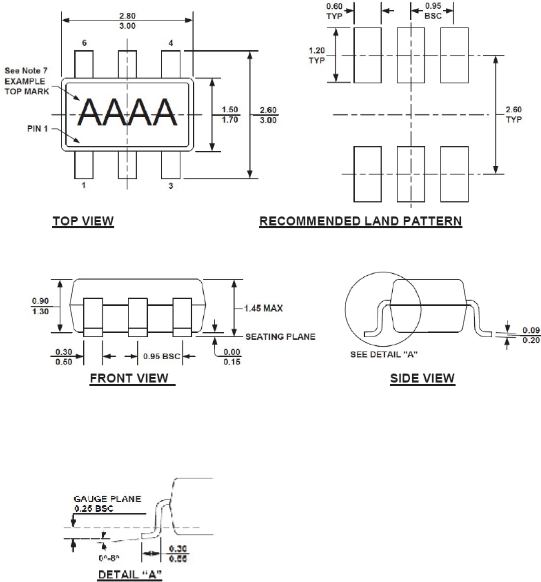
Figure 9. TSOT23-8/SOT23-6 Physical Dimensions
