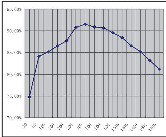
Vin=5V, Vout=1.8V
