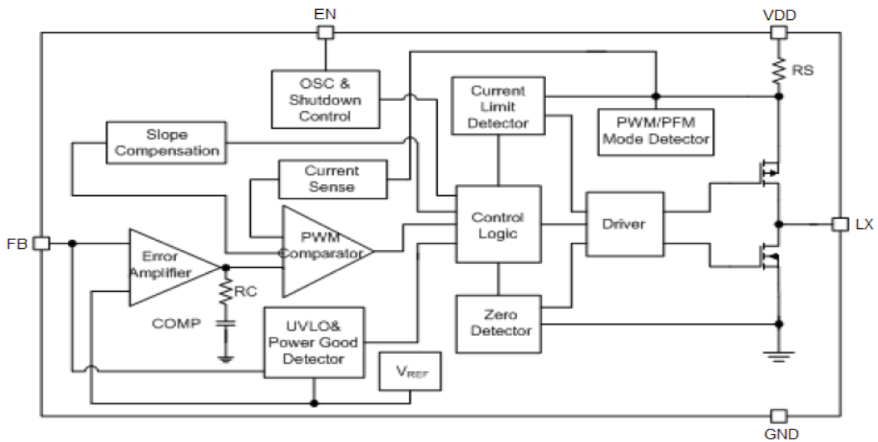
Figure2 TCS4205 Block Diagram
